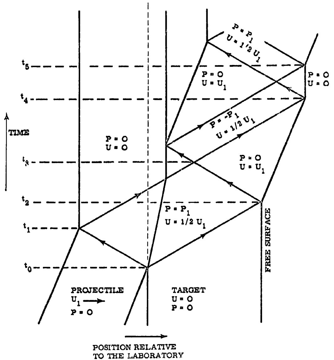
Figure 2. Wave Diagram of a Single Shock Wave Produced by a Low Velocity Impact of Two Plates of the Same Medium
