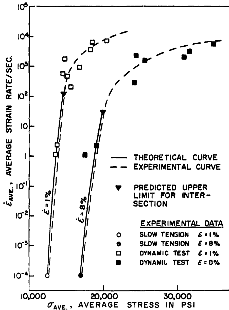
FIG. 6 PREDICTION OF THE DYNAMIC PLASTIC BEHAVIOR IN THE INTERSECTION REGION FOR PURE Al AT T = 77^\circ K .
