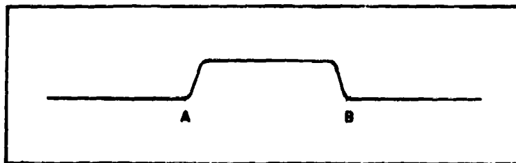
FIGURE 6. DISLOCATION ENERGY
