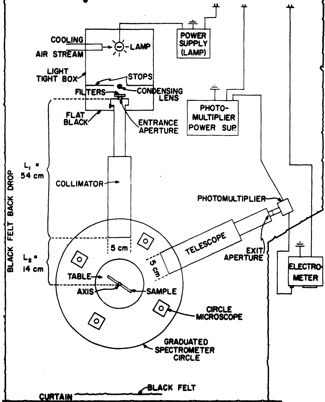
Figure 1. Schematic Diagram of Photometric Equipment.
