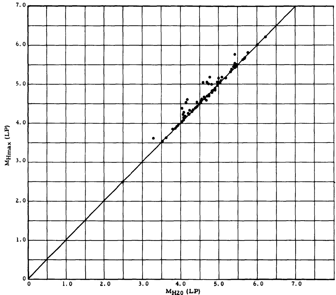
Figure 31. M_{Hmax} as a function of M_{H20} for 102 earthquakes recorded at WMSO 1 March-31 May 1962
