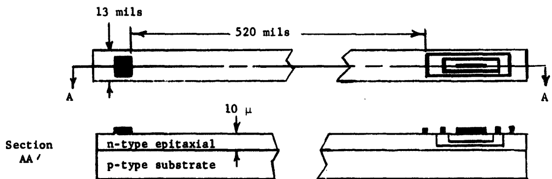
(b) Fabrication of R_1 in 1 ohm-cm n-type Epitaxial Layer
