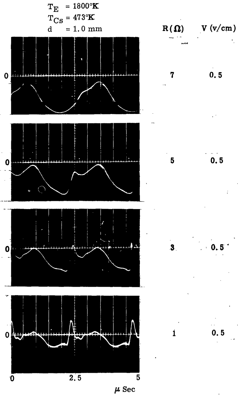
Figure 34. Oscillation Data for High Resistance Load
