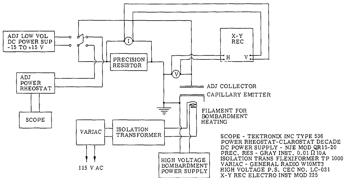
Figure 3. Converter Measurement Circuit
