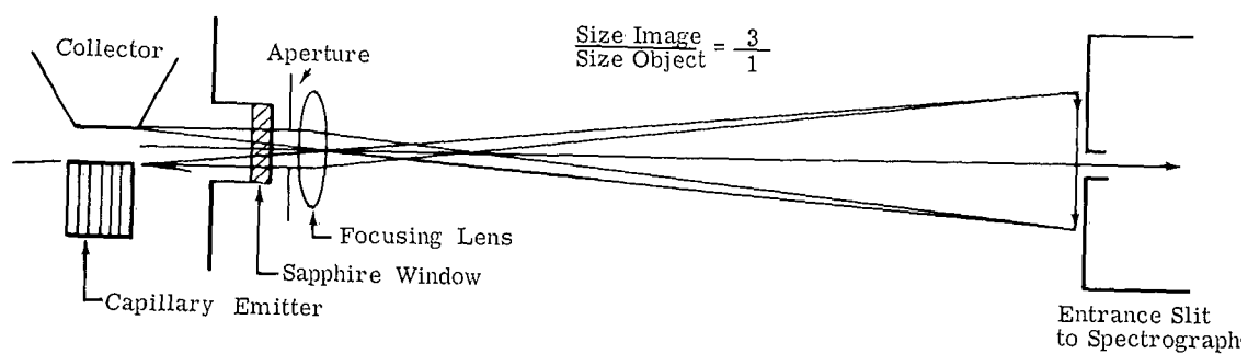
Figure 37. Spectrographic Arrangement
