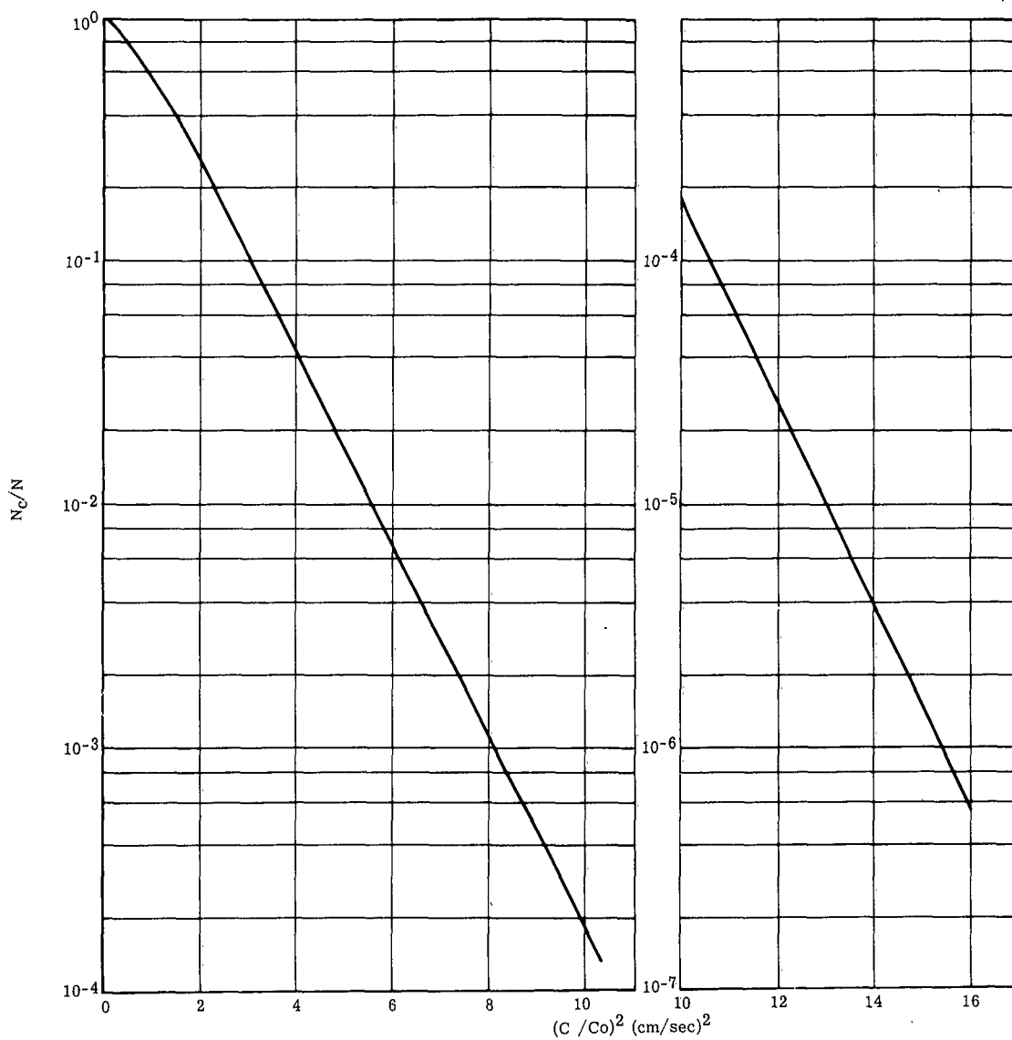
Figure 39. Fraction of Electrons Above a Given Energy in a Maxwellian Distribution
