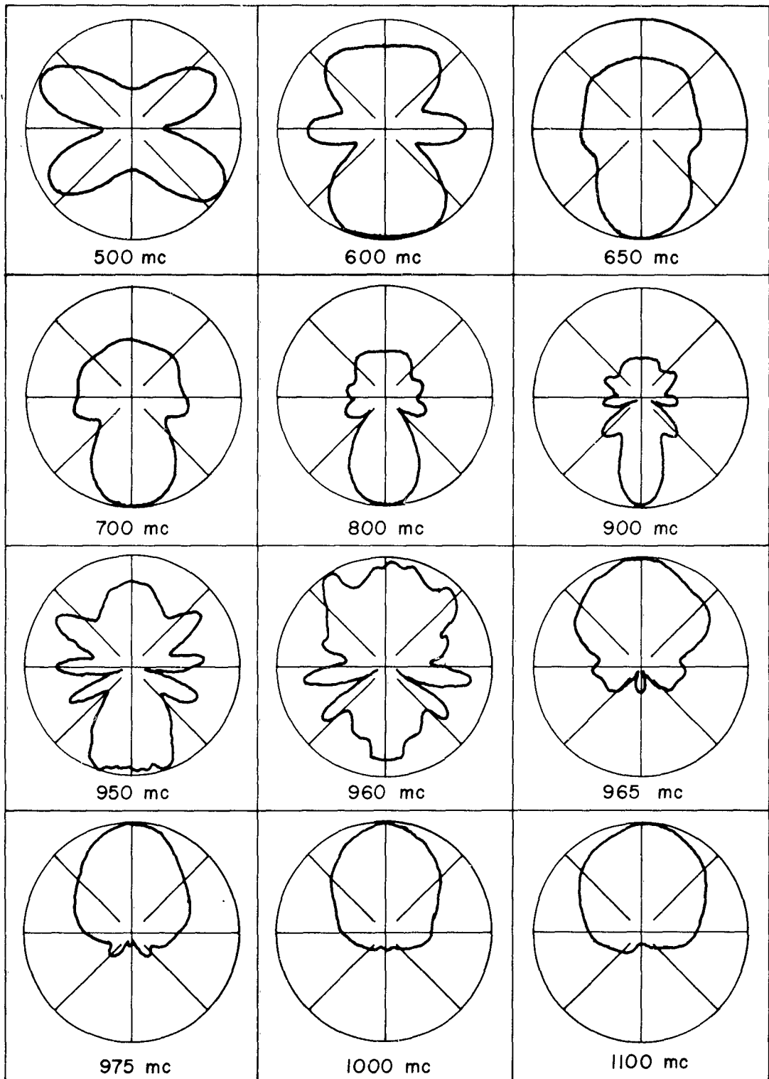
Figure 52. Measured H-Plane Voltage Patterns for HFUPM(5).
