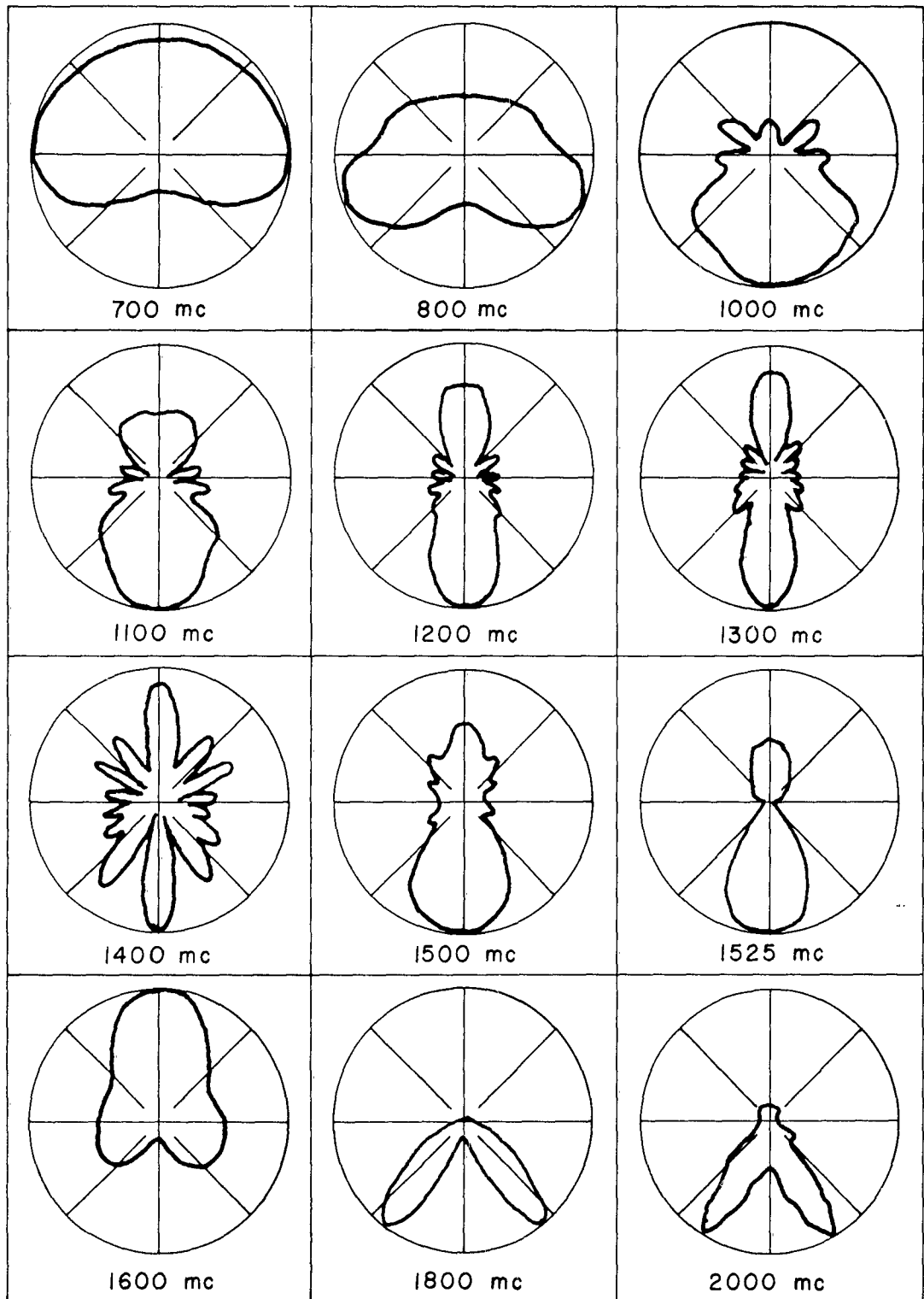
Figure 20. Measured H-Plane Voltage Patterns for UPM(2)A.
