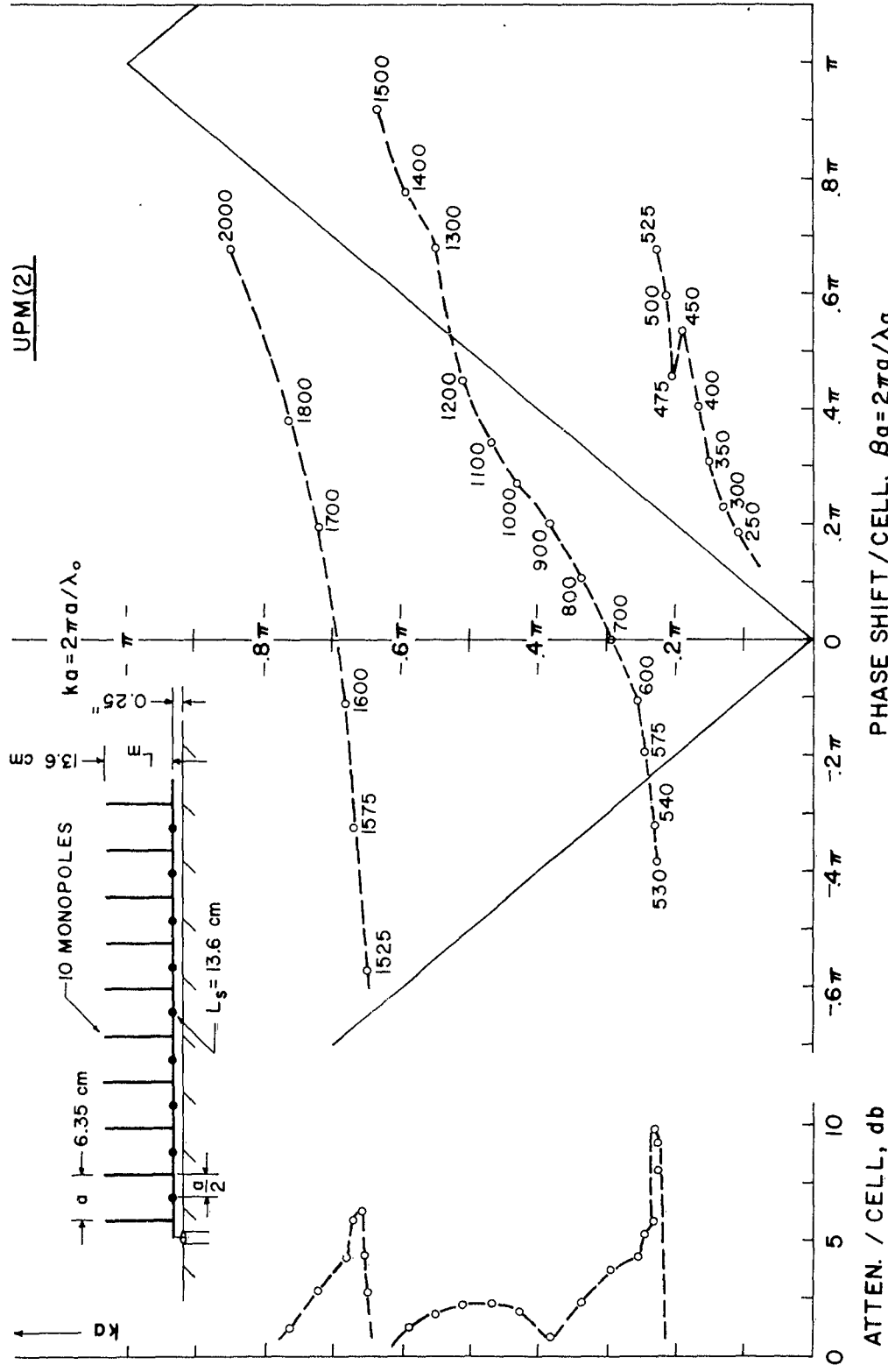
Figure 21. The k - \beta / Attenuation Diagram for the Stub-Loaded Monopole Array, Type-I. UPM(2).
