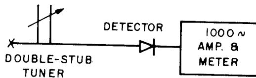
Figure 8. Details for Measurement of Approximate Front-to-Back Ratio.
