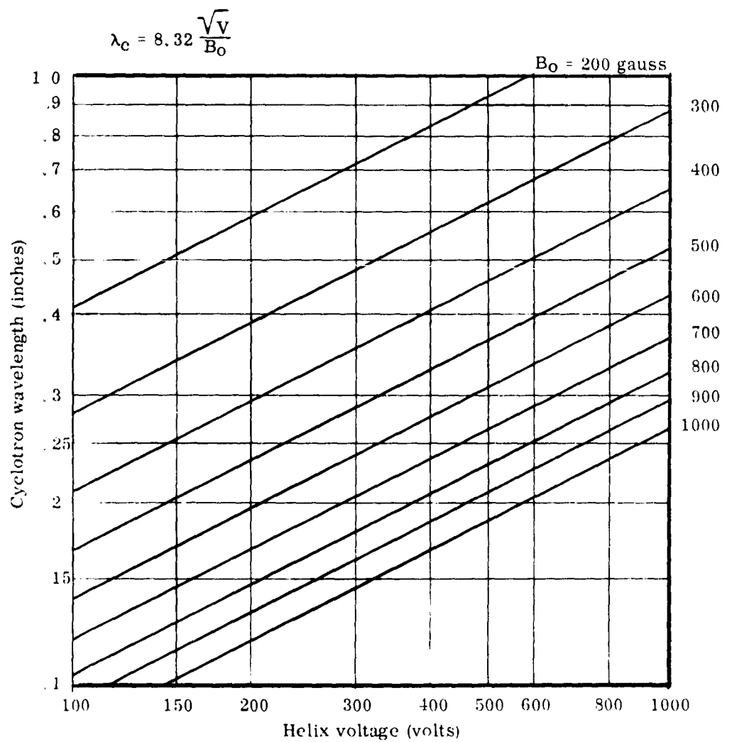
Fig. 7 - Cyclotron wavelength vs beam voltage, with magnetic field as a parameter. For low space charge, the cyclotron wavelength is the same as the scalloping wavelength of the beam.
