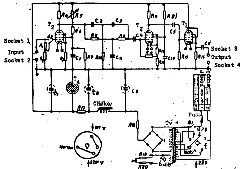
Fig. 3. Schematic diagram of AZ-2 amplifier.
