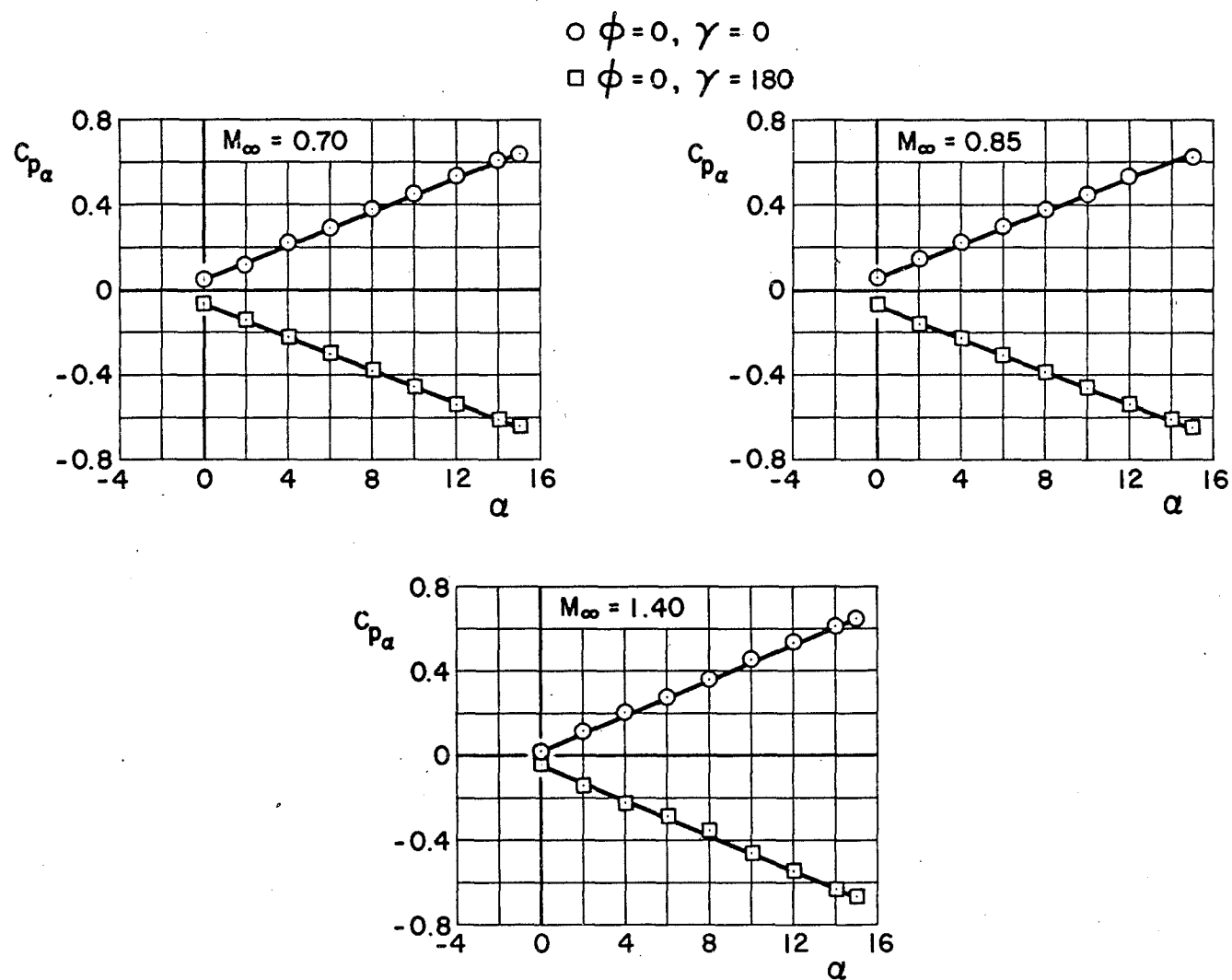
d. Probe One of Eight-Probe Configuration
