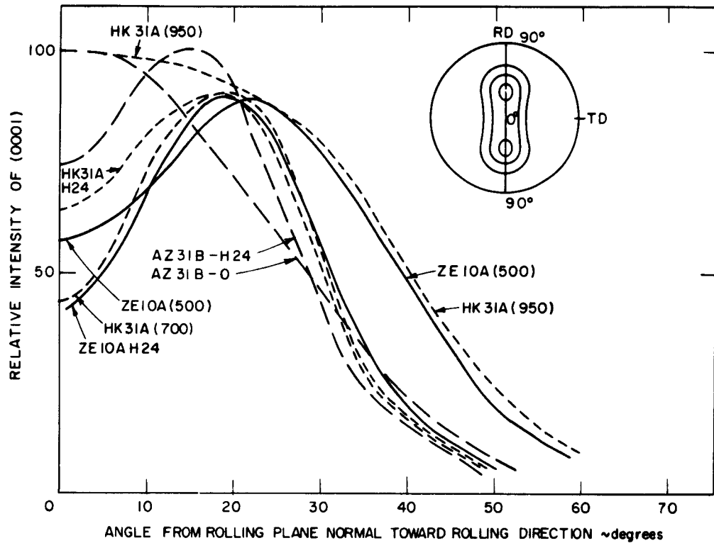
Figure 5. Profiles of (0001) pole figures for the magnesium alloy sheets showing the rolling direction spread of the intensity of (0001) reflections. The curves are the average of the intensities along great circles from the rolling plane normal to both the positive and reverse rolling directions as indicated at upper right.
