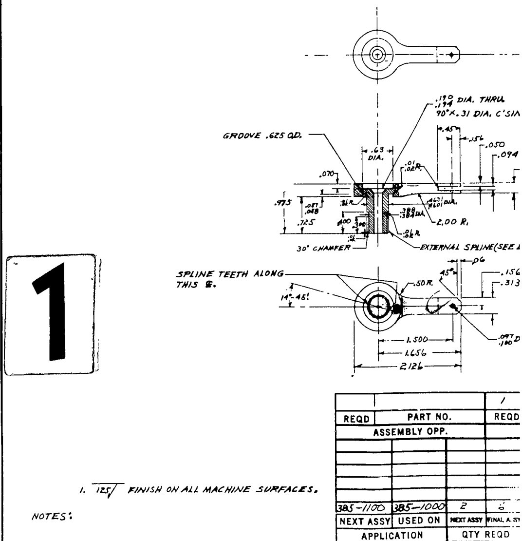
Figure 6. Aft Duct Lever.
