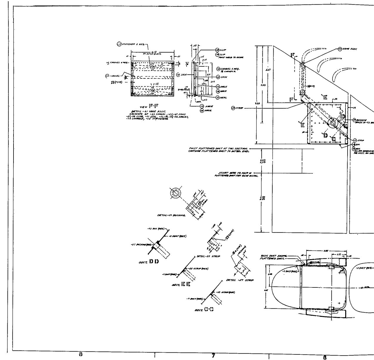
Figure 2b. Tip Assembly, Sheet 2.
