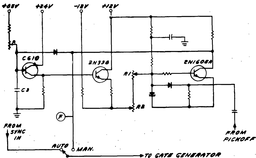
Figure 12. Variable Delay
