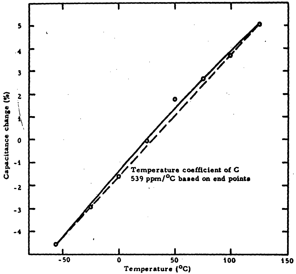
Fig. 24. Percentage capacitance change at 1 kc relative to room temperature value as a function of temperature for an aluminum capacitor.
