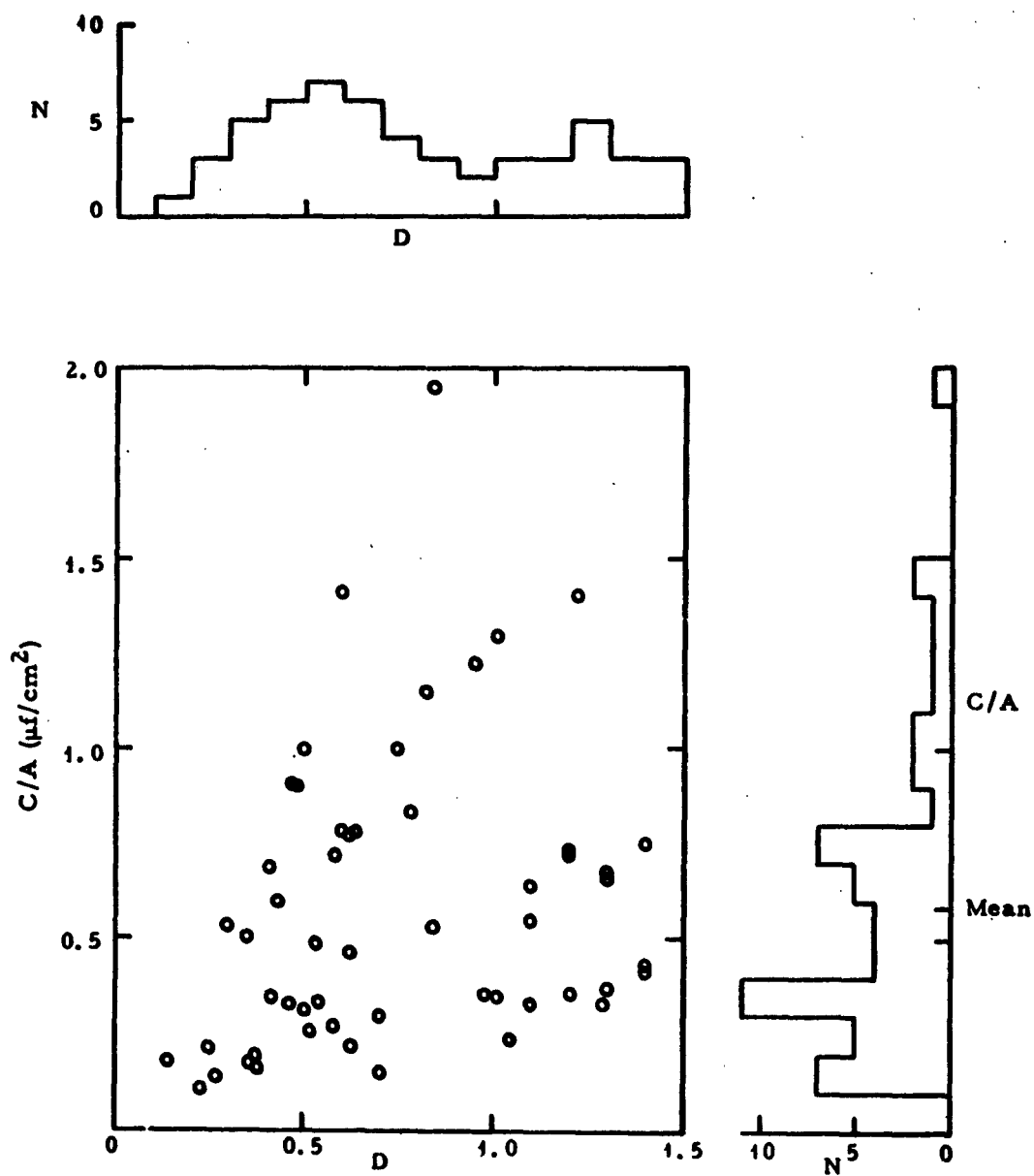
Fig. 37. Capacitance per unit area vs dissipation factor, and their numerical distributions for tungsten anodized in sulfuric acid at 50 volts.
