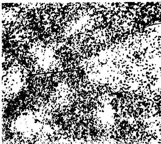
Fig. 27 95 Nb 5 Sc annealed 113 hrs. at 1200 °C
