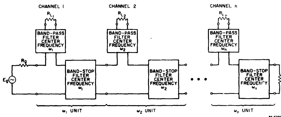
FIG. II-1 SCHEMATIC REPRESENTATION OF A MULTIPLEXER OF A PARTICULAR DESIGN
