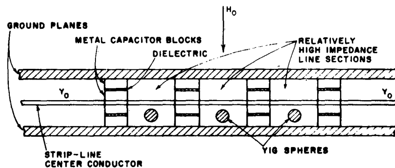
FIG. III-5 A SUGGESTED MAGNETICALLY TUNABLE BAND-STOP FILTER CONFIGURATION THAT PERMITS INCREASED COUPLING TO THE YIG SPHERES
