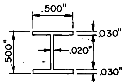
(c) APPROXIMATE SECTION (PHOSPHOR BRONZE)
