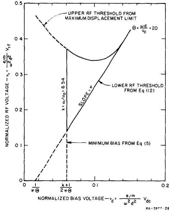
FIG. 6 ILLUSTRATION OF THE UPPER AND LOWER RF THRESHOLD AND MINIMUM BIAS FOR ONE-SIDED MULTIPACTOR DISCHARGE
