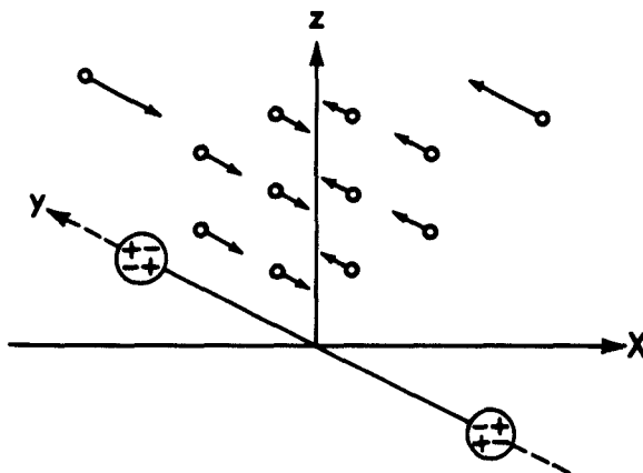
Fig. 13. Field in quadrupole midplane.
