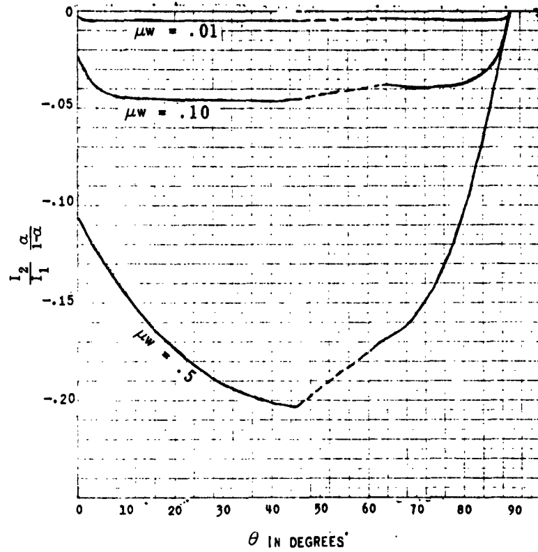
Fig. 4. (I_2/I_1) \frac{a}{1-a} versus \theta for a range of values of \mu_w = 0.01-0.5 corresponding to the range of effective particle size from fine to coarse, respectively. The dashed line was obtained by interpolation.
