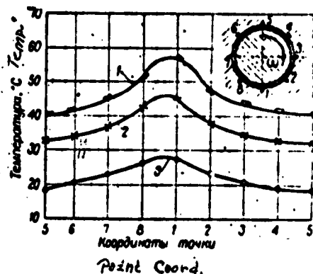
Fig. 5. Curves showing temperature distribution along the perimeter of the bearing at specific pressures; 1- 24.6 \text{ kg/cm}^2 ; 2- 17.2 \text{ kg/cm}^2 ; 3- 8.8 \text{ kg/cm}^2 .
