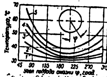
Fig. 8. Temperature dependence curves of most heated zone upon angle of lub feeding ( p ) and specific pressure p : 1-4.4 \text{kg/cm}^2 ; 2-6.9 \text{kg/cm}^2 ; 3-8.3 \text{kg/cm}^2 ; 4-11.2 \text{kg/cm}^2 ; 5-13.8 \text{kg/cm}^2 .
