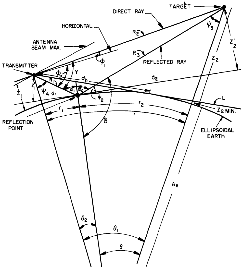
Figure 1. Ray Representation of Propagation in the Interference Region Above A Curved Earth
