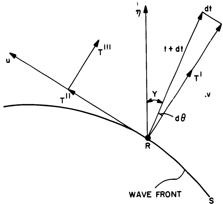
Figure 8. A Vector Analysis of a Wavefront
