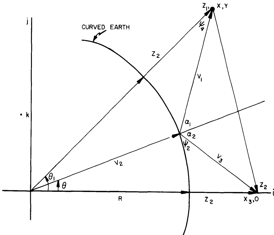
Figure 2. Vector Representation of Interference Region
