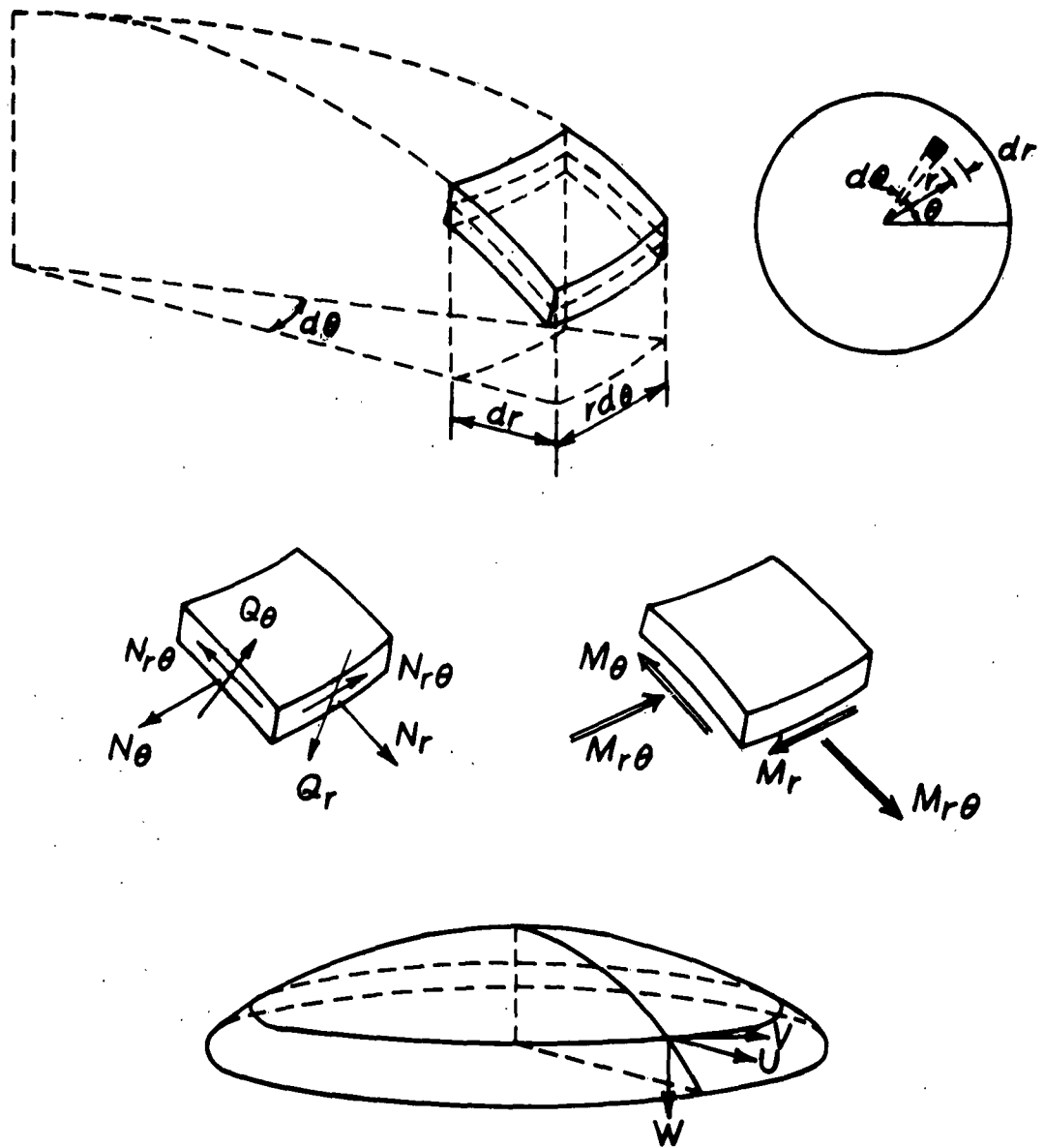
FIG. 4 STRESS RESULTANTS, MOMENTS AND DISPLACEMENTS IN SHELLS
