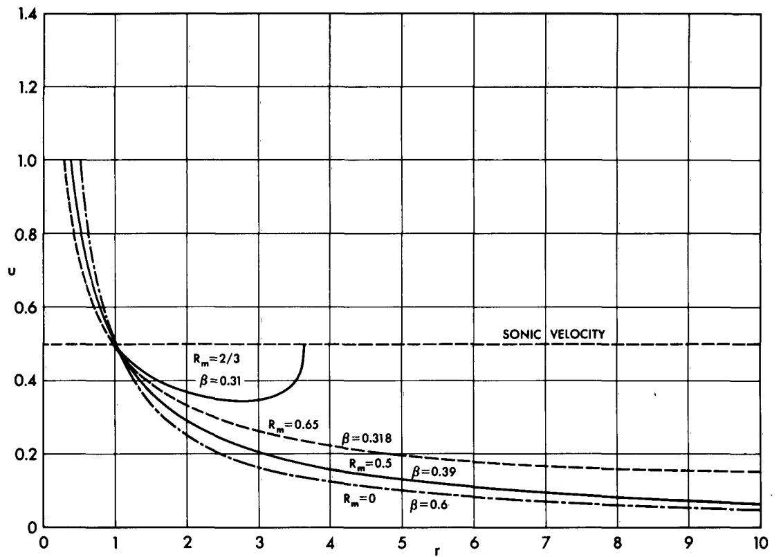
Fig. 29. Velocity distribution. r_c = 1 and \left(\frac{du}{dr}\right)_c from region I of Figure 28. Case 5.
