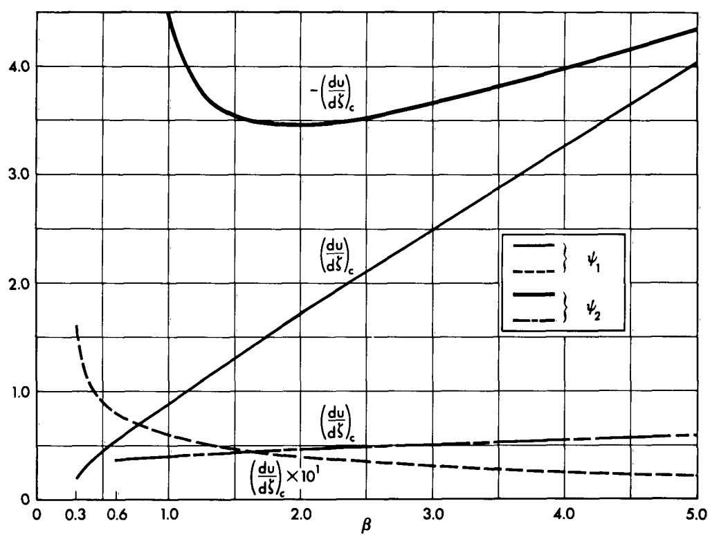
Fig. 8. Variation of (\frac{du}{d\xi})_c with \beta . Case 4, E < 0 .
