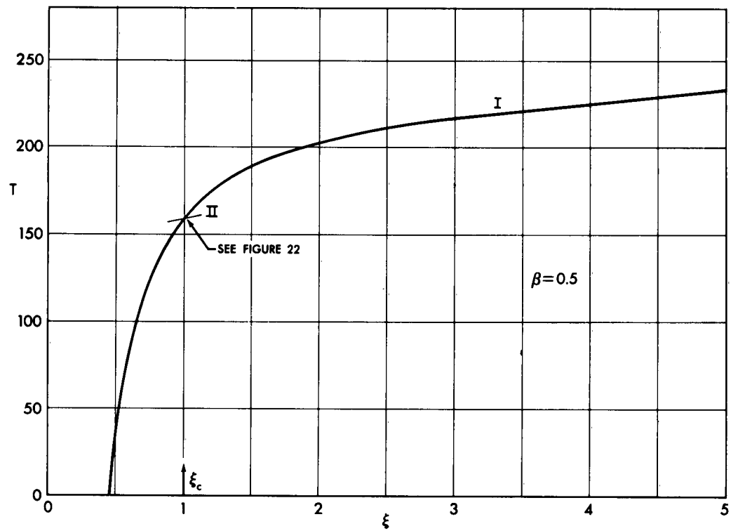
Fig. 17. Variation of T with \xi for \zeta_c = 1 and \beta = 0.5 . Case 4, E > 0 .
