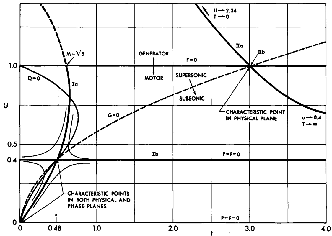
Fig. A-2. Solution of constant area channel in the phase plane.
