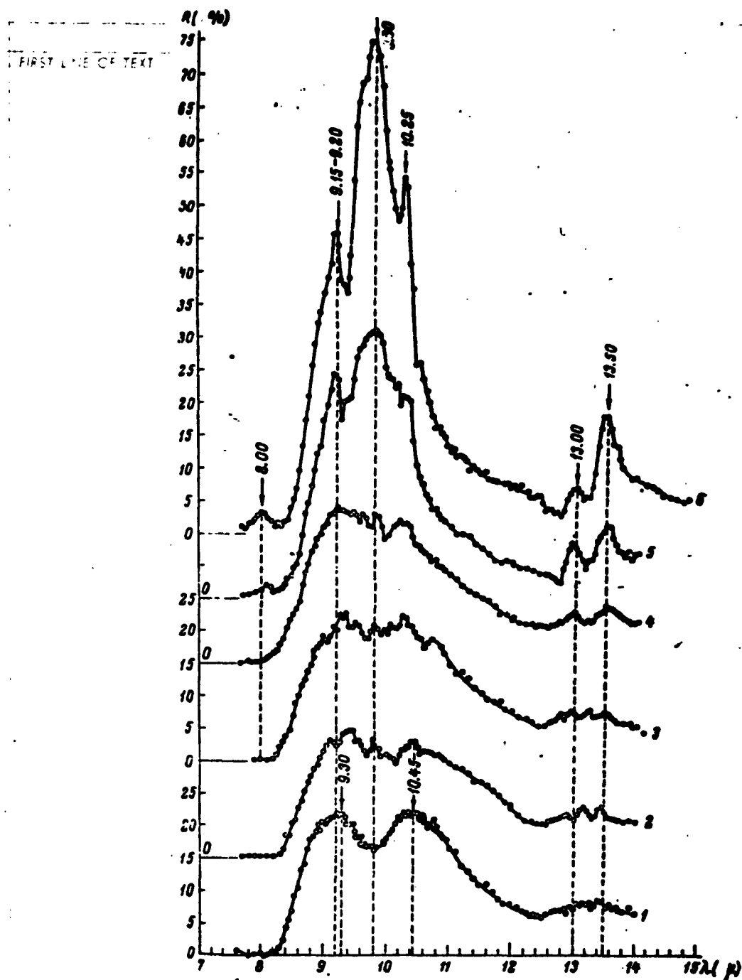
Fig. 6. Reflection spectra of glass with 30% \text{Na}_2\text{O} and 70% \text{SiO}_2 . 1) initial glass; 2) crystal part of rich glass heated at 610-620^\circ , \tau = 1 hr; 3) the same, \tau = 3 hrs; 4) the same, \tau = 6 hrs; 5) crystal part of crystallized glass heated at 610-620^\circ , \tau = 12 hrs; 6) the same, \tau = 72 hrs.
