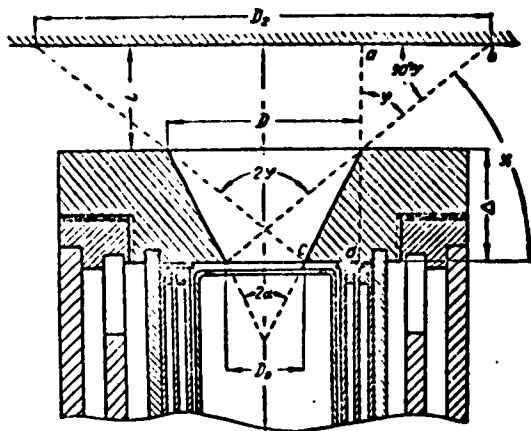
Figure 7. For determining the distance from the radiation thermometer to the emitter:
