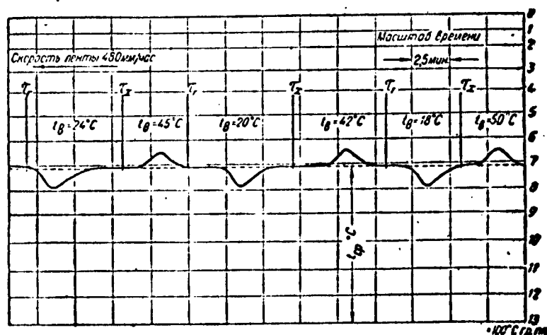
Figure 6. The effect of the intensity of cooling on the readings of a radiation thermometer: t_w - water temperature; t_{av} - average steady value of the thermometer readings; \tau_x \tau_r - moment when water temperature was varied.
