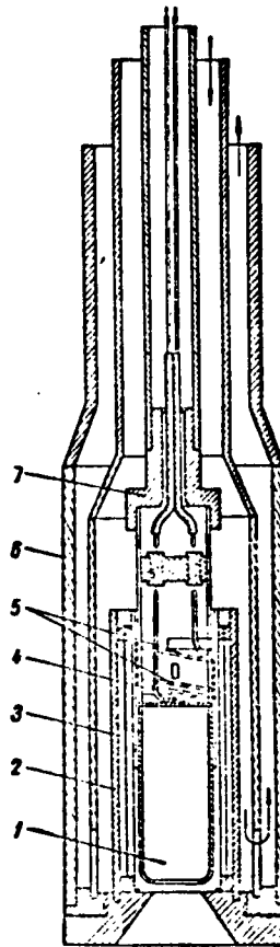
Figure 2. Structure of the radiation thermometer: 1 - heat receptor; 2 - protective jacket; 3 - shielding; 4 - thermopile; 5 - heat resistors; 6 - water-cooled body; 7 - sleeve.
