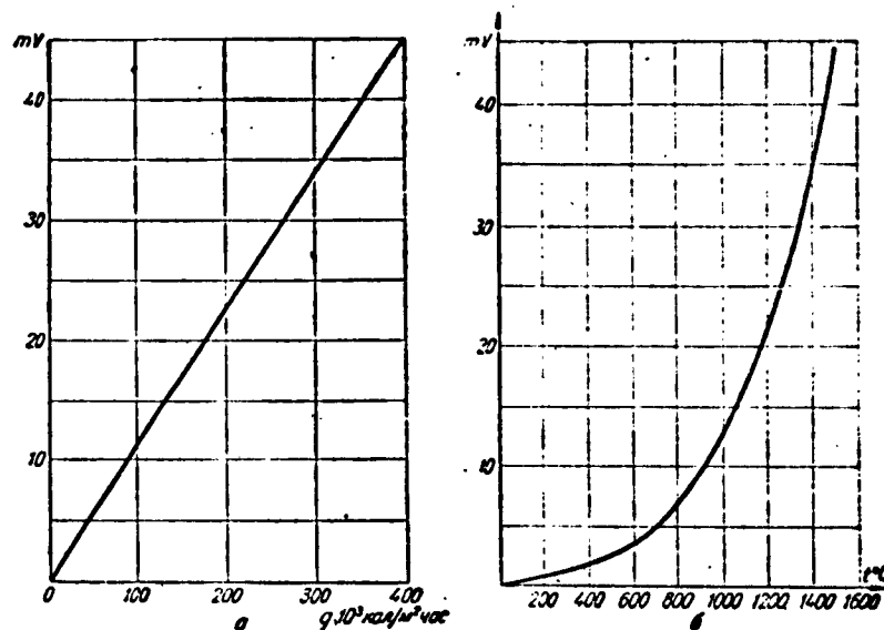
Figure 4. Response of the radiation thermometer: a - by heat flow; b - by temperature.
