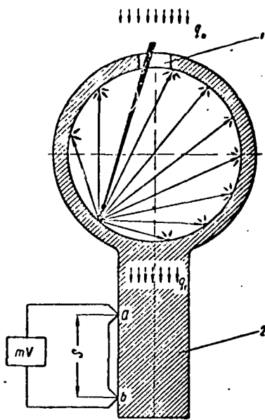
Figure 1. Diagram of the measuring element of the radiation thermometer: 1 - heat receptor; 2 - cooled shank.
