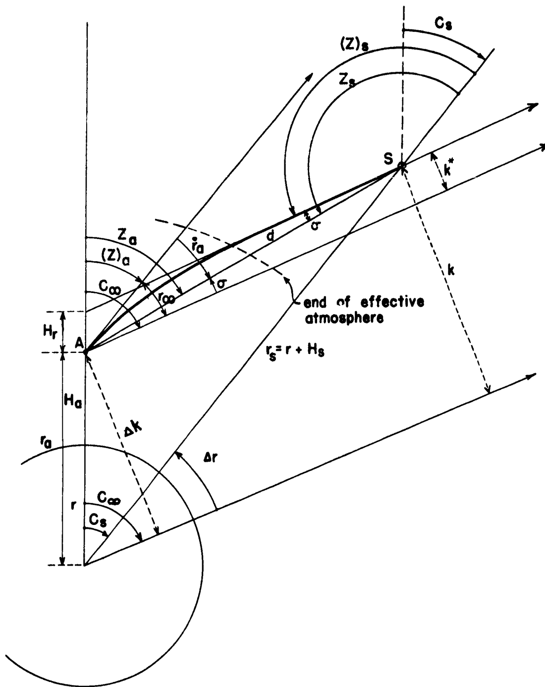
Classic refraction geometry.
