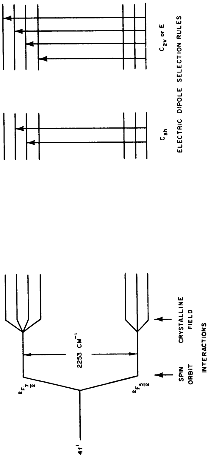
FIGURE 1. Energy Levels and Electric Dipole Selection Rules for Ce^{3+} in LaF_3
