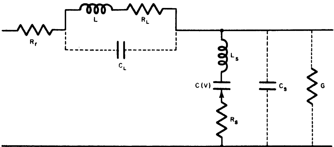
FIGURE 2. Equivalent Circuit
