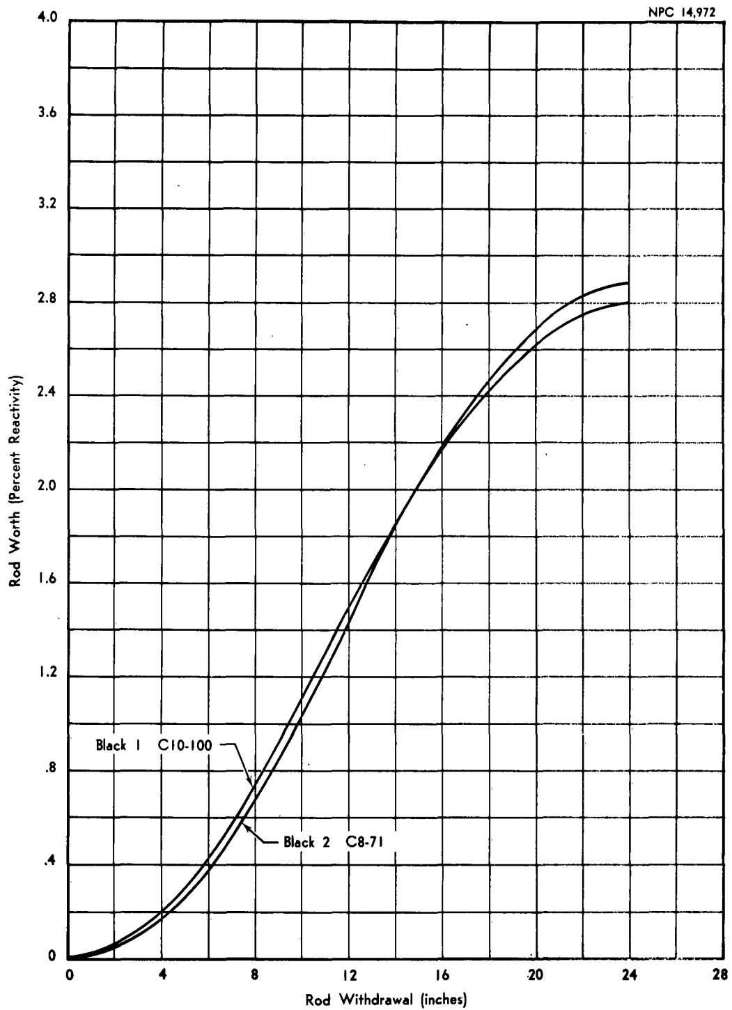
Figure 10. Shim-Safety-Rod Calibration
