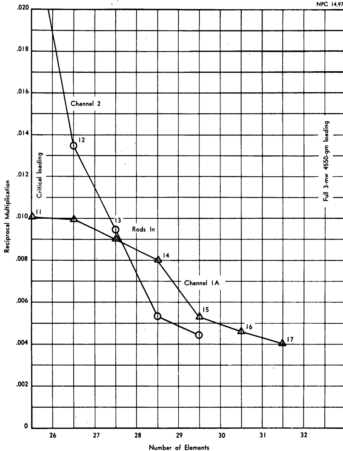
Figure 8. Channels 1A and 2 Loading Adjustment Reciprocal Multiplication Curve
