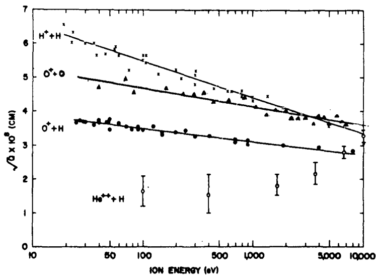
Fig. 8--Cross sections for the symmetrically resonant charge transfer collisions between H^+ and H, and between O^+ and O. The accidentally resonant process between O^+ and H is seen to display the characteristics of resonant charge transfer over the energy range in this figure, but the process He^{++} + H \rightarrow He^+ (n=2) + H^+ does not. The data are from reference 15
