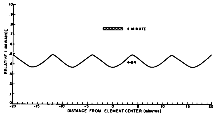
Fig. 43. Luminance cross-section of Ball-bearing Board Background showing the location of the 4 minute target centered between the elements.
