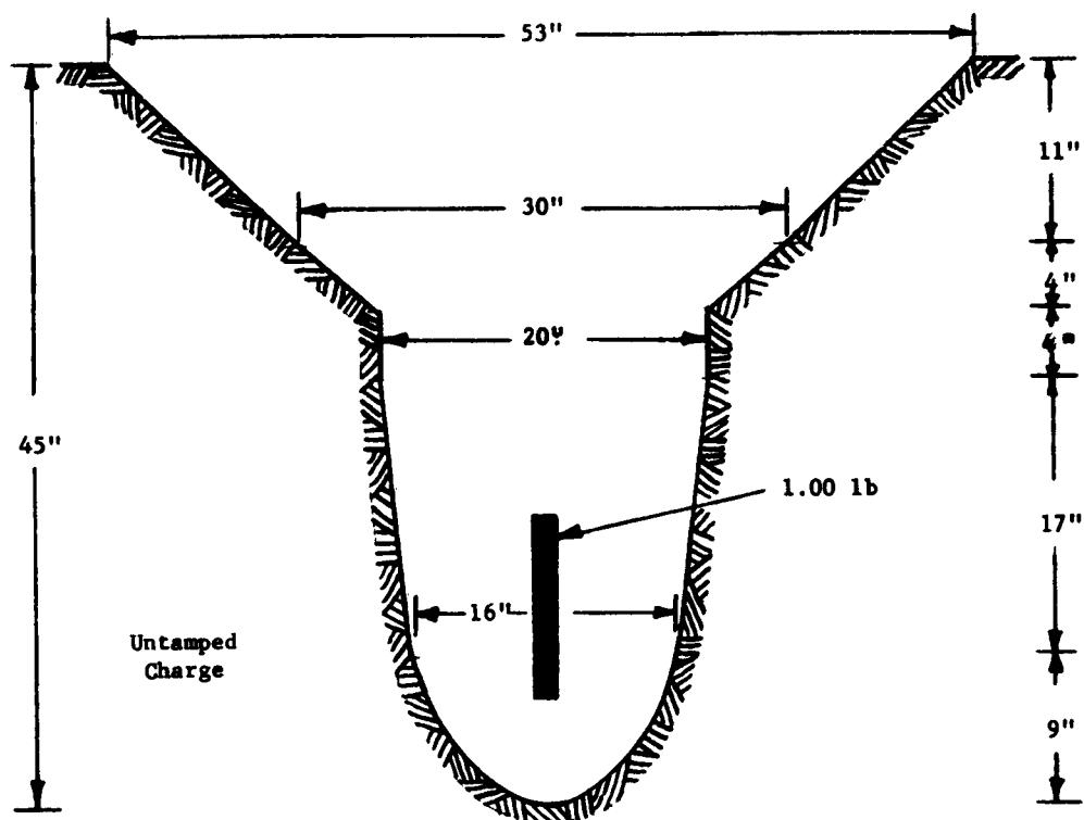
Cleaned Crater Profile, Charge 81
