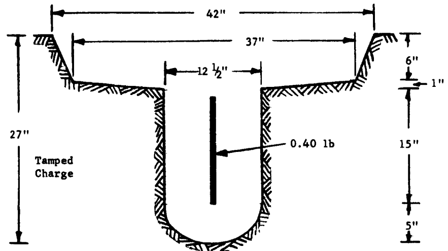
Cleaned Crater Profile, Charge 22
