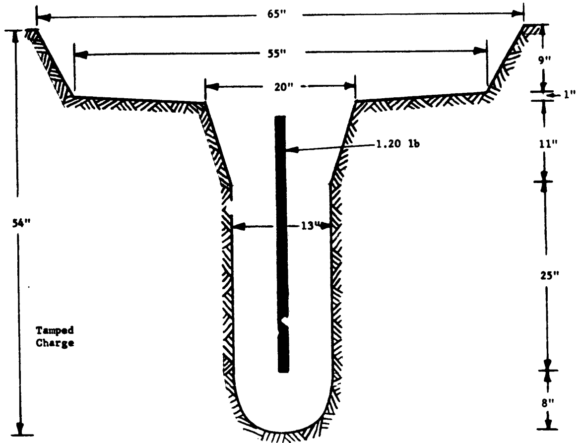
Cleaned Crater Profile, Charge 49
