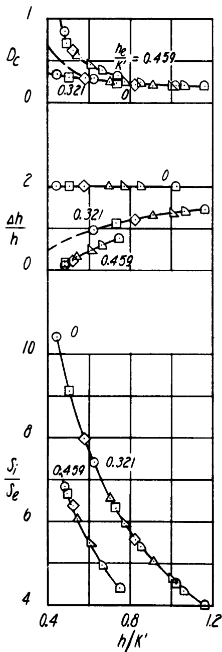
Figure 14 - Variation of the Parameters D_c , \Delta h/h , and S_i/S_e With h/k' for Several Values of h_e/k' . \theta = -75^\circ (a) \frac{S}{S_1} = 5.27
