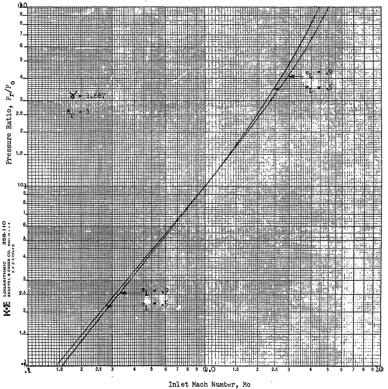
Pressure Ratio versus Inlet Mach Number
