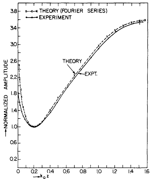
FIG. 1-6 COMPARISON OF THEORETICAL AND EXPERIMENTALLY DETERMINED CURRENT DISTRIBUTION (AMPLITUDE) k_0 h = \pi/2 ; \sigma_\lambda = 0.0105 ; M = 10
