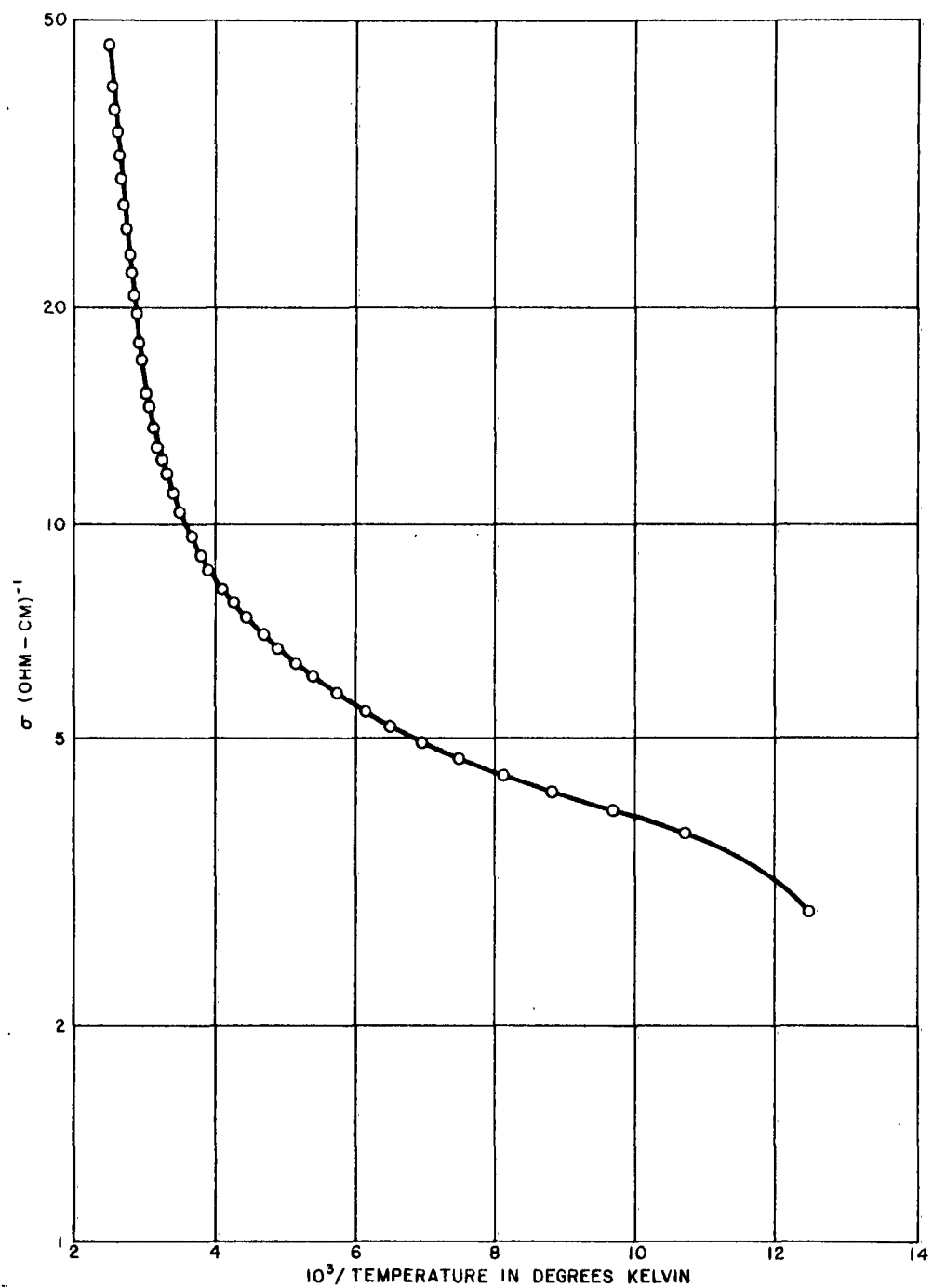
FIGURE 3. Dependence of the Electrical Conductivity Upon the Reciprocal Absolute Temperature at Zero Magnetic Field for a Cu-Doped InSb Film
