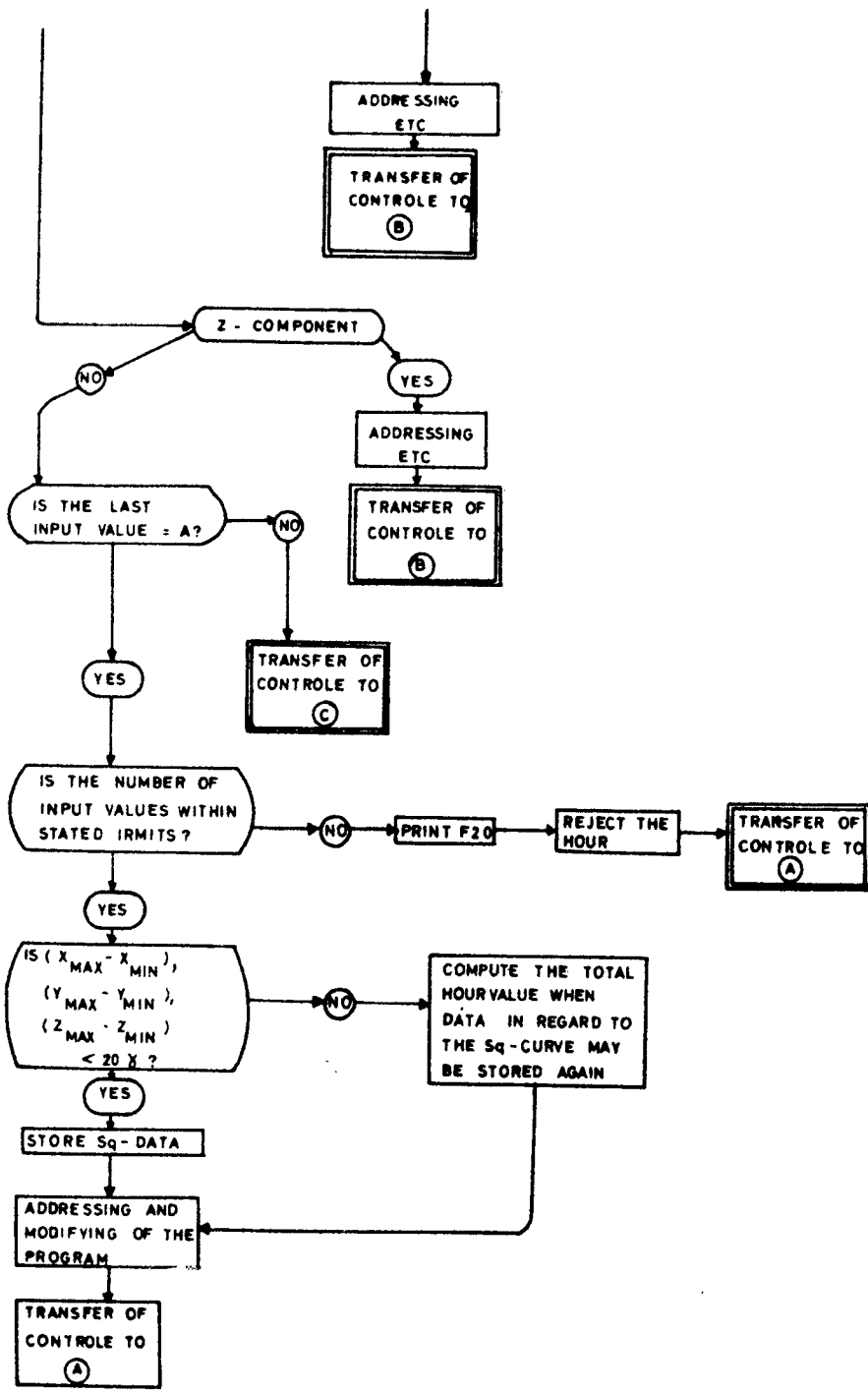
FIG 8. Abridged flow diagram, part 2.
