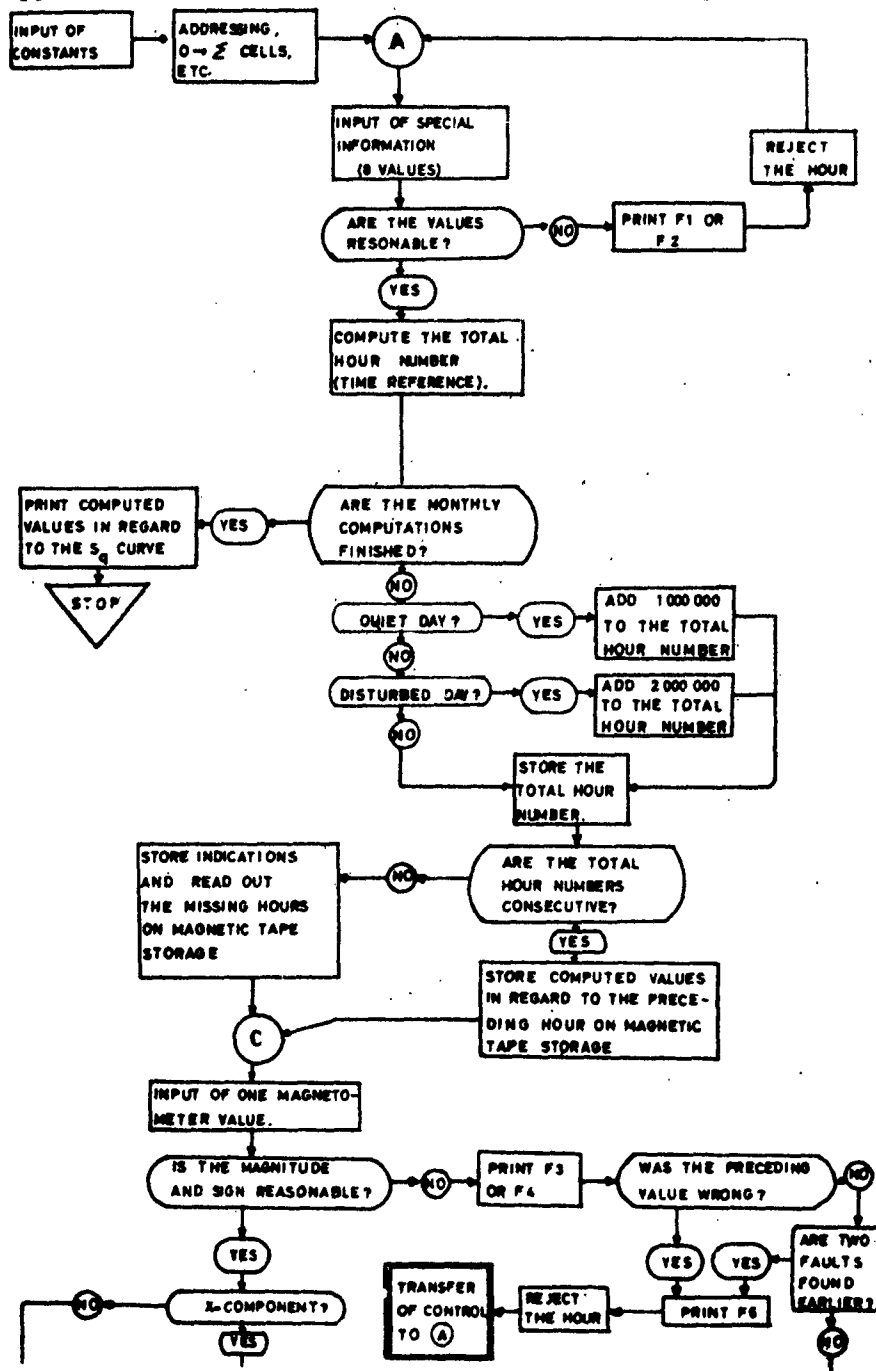
FLOW-DIAGRAM. COMPUTER-EDITING OF MAGNETOMETER-VALUES.
