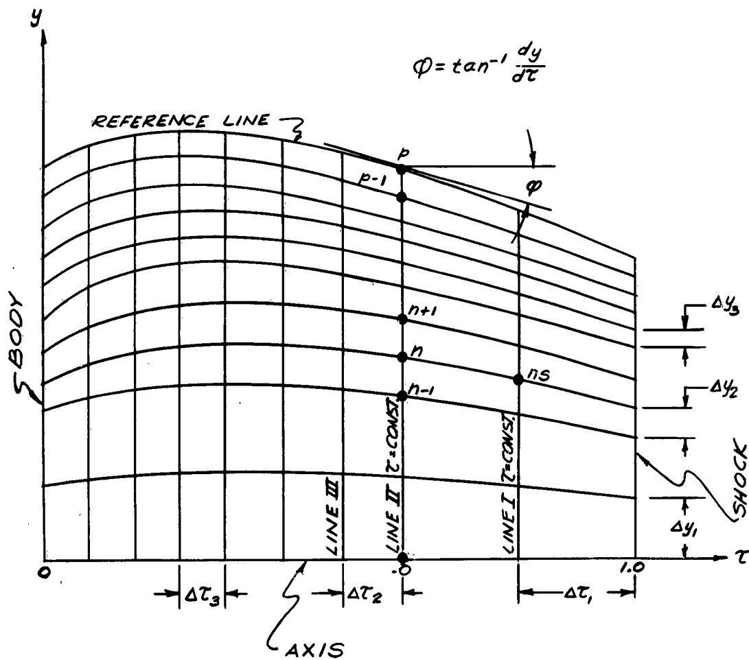
FIG. II TRANSFORMED \tau - y PLANE SUBSONIC REGION
