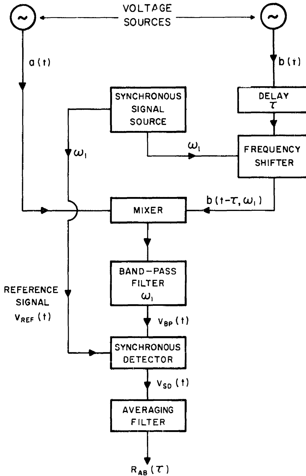
Figure 2. The Cross-Correlator.
