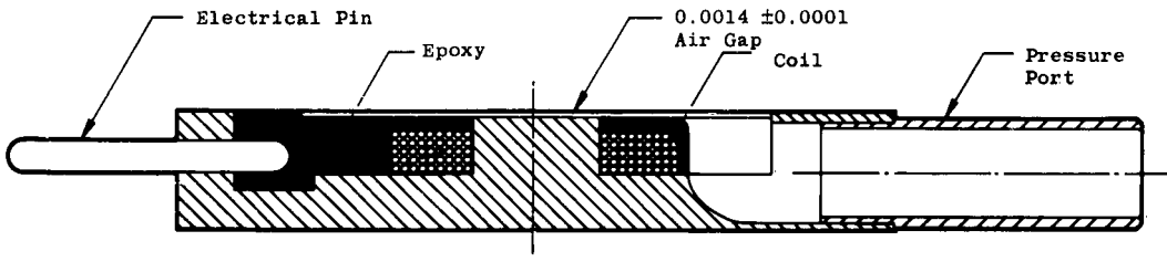
Fig. 15 Wafer Gage with Machined Potting
