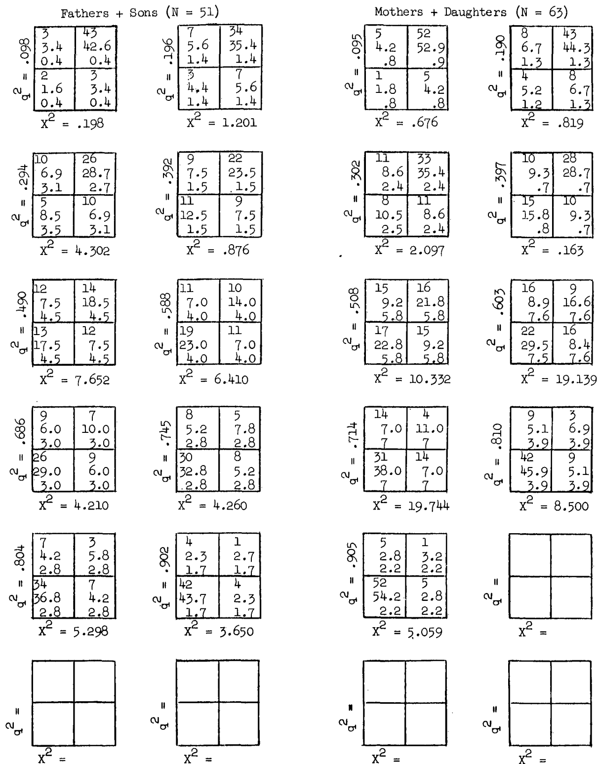
FIG. D-1. SYMBOL COMPARISON TEST. Hypothetical Dichotomies and Chi-square Tests of Goodness of Fit (Low Score = Recessive)
