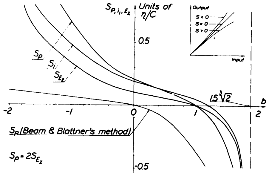
Fig. 5. Depicting the amplitude nonlinearity parameters S_{E,i,p} versus the electron velocity parameter b .
