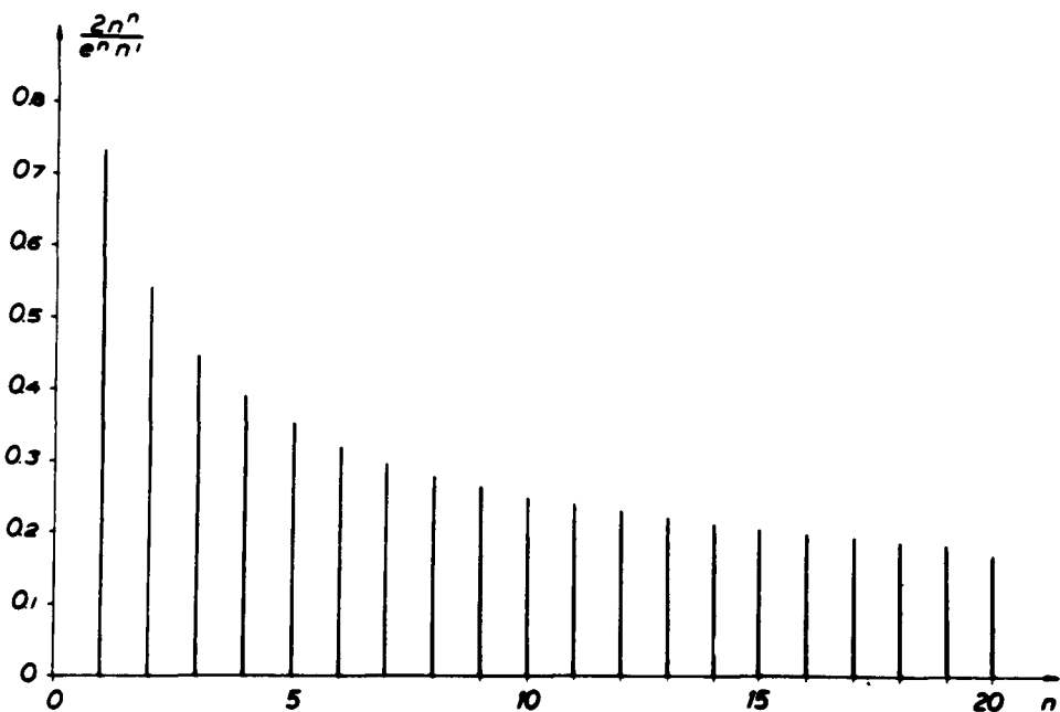
Fig. 12. The amplitudes of the normalized ac harmonic electron current waves, \frac{(nR)^n}{n!} \left(\frac{1}{2}\right)^{n-1} at the limit of convergence of Eq. (81), i.e. for R = 2/e .
