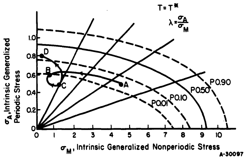
FIGURE 18. TIME TRAJECTORY OF A SYSTEM PLOTTED ON A GENERALIZED STRESS-RANGE DIAGRAM
