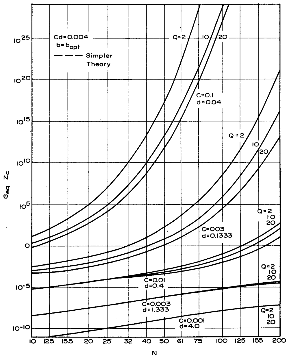
Figure 11. Dependence of Equivalent Conductance on Circuit Length. Cd = 0.004 , b = optimum value for each C, N, Q .
