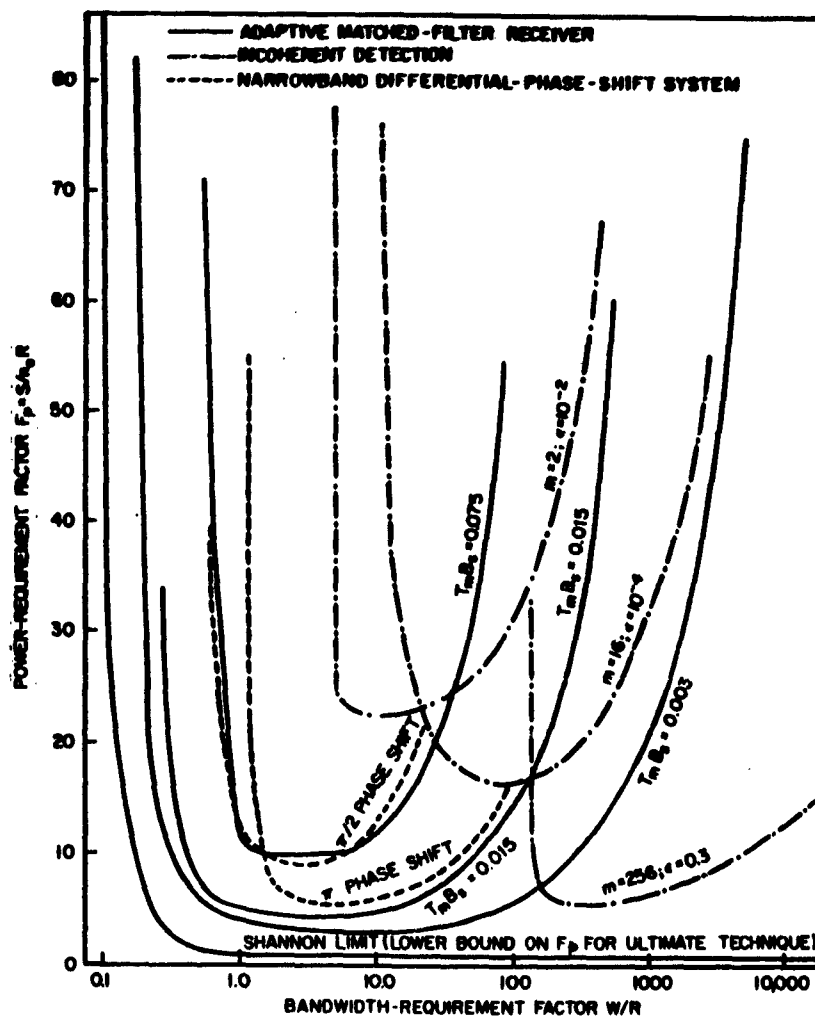
FIG. 15. POWER REQUIREMENTS VS BANDWIDTH REQUIREMENTS.
