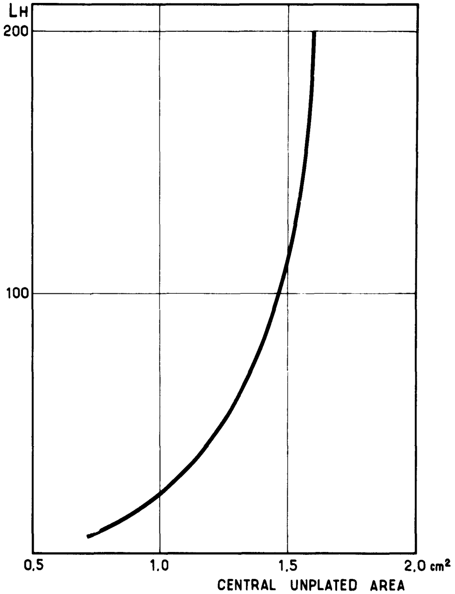
L FIELD L AS FUNCTION OF CENTRAL UNPLATED SURFACE. Fig. 5
