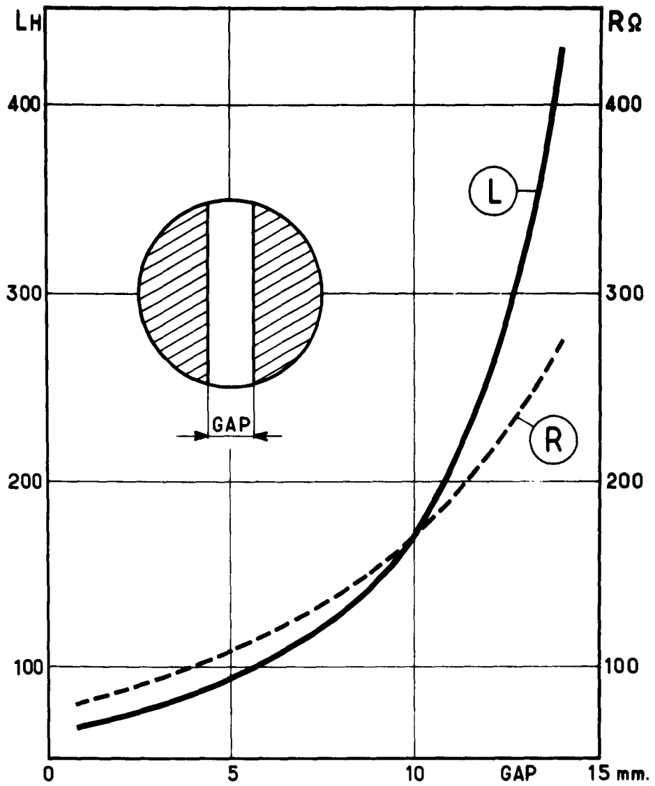
// FIELD L AND R AS FUNCTION OF THE GAP. Fig. 1
