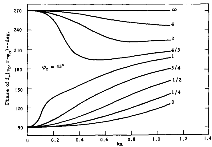
Graph III-3(b)
