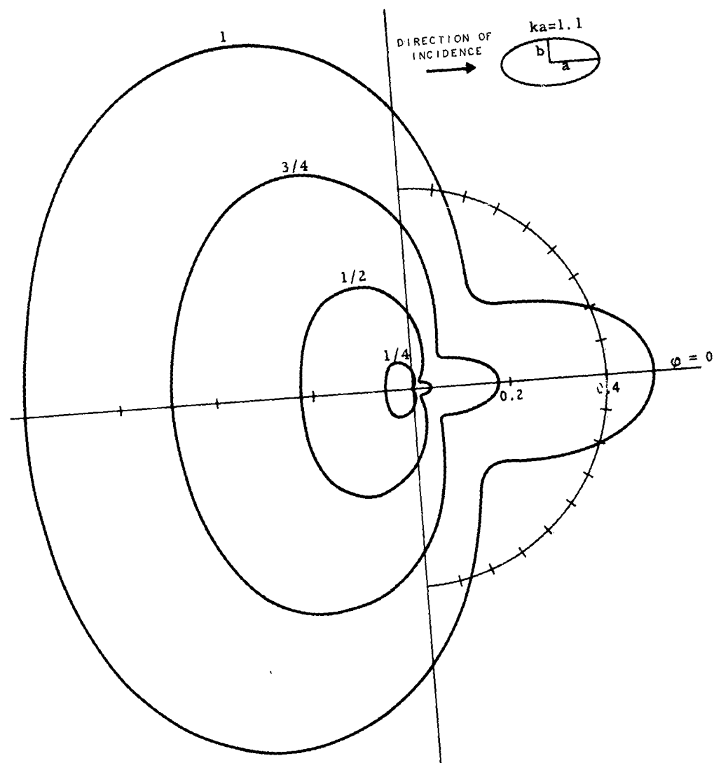
Graph I-10(a): |g_+(\varphi, 0)|^2 .
