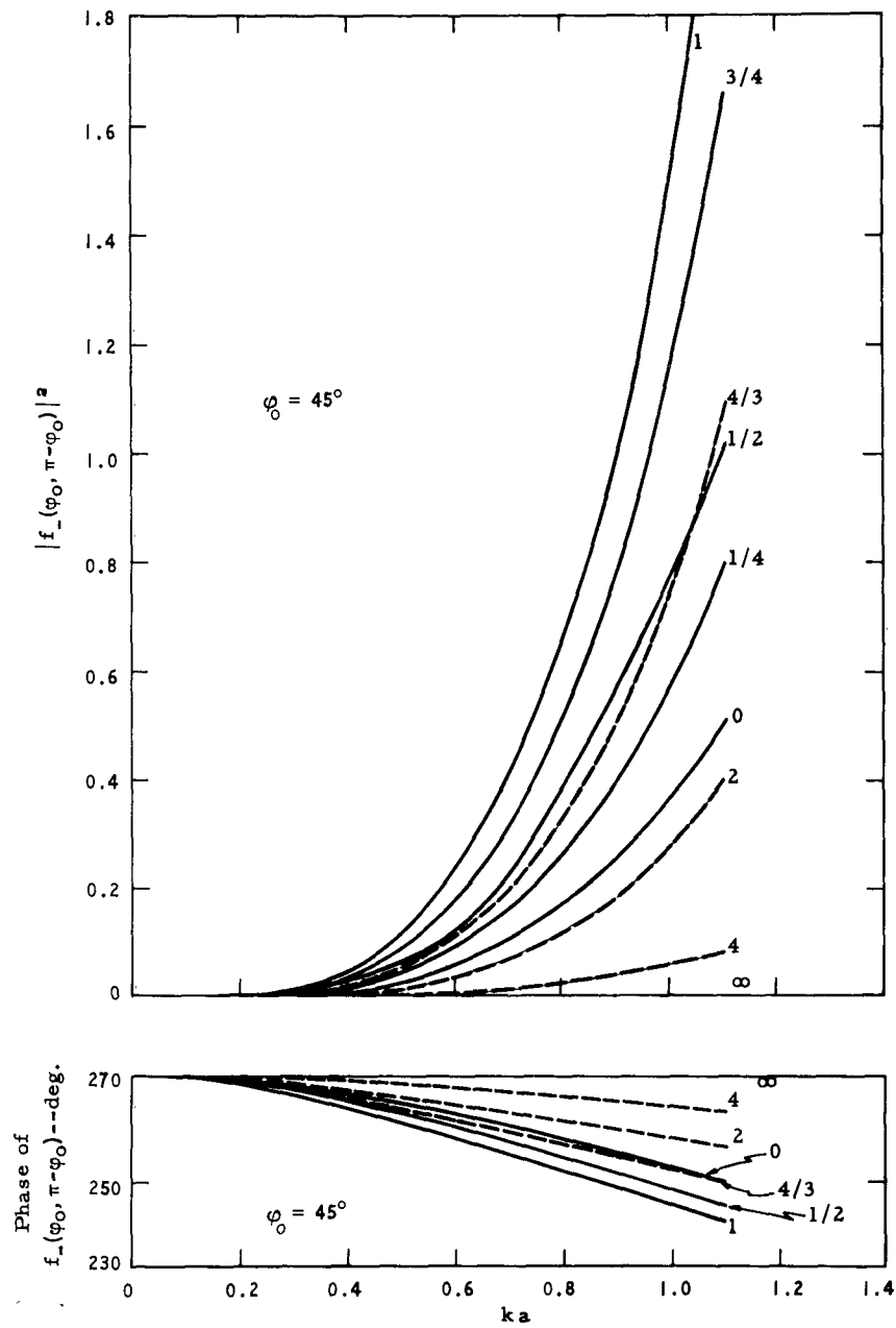
Graph IV-3(b)
