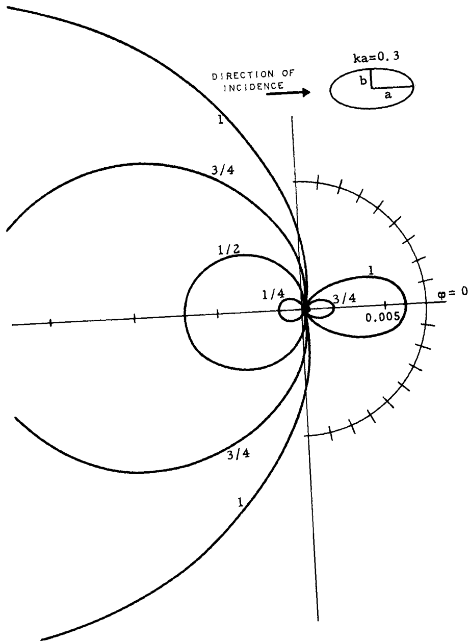
Graph I-6(a): |g_+(\varphi, 0)|^2 .
