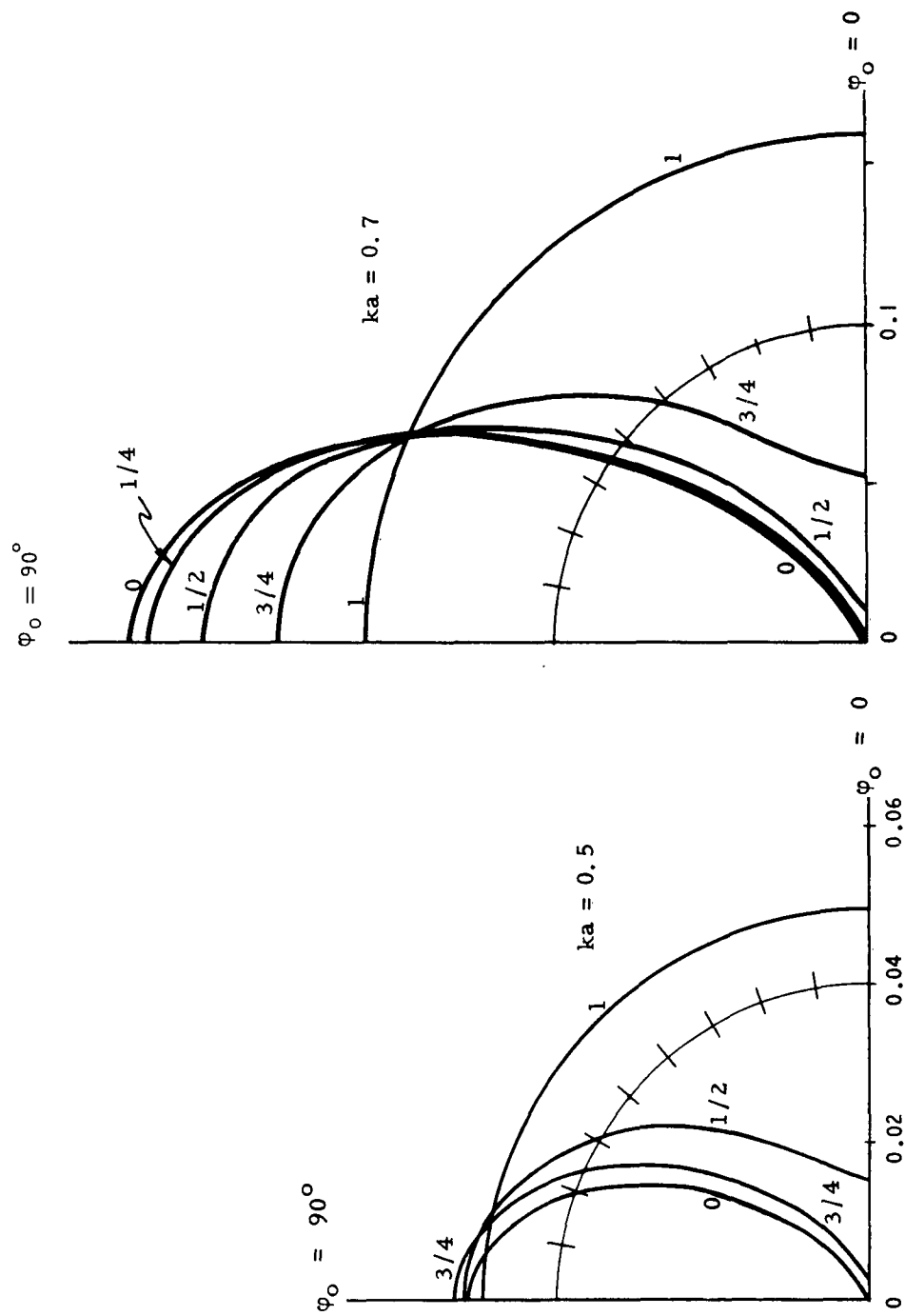
Graph I-2: |g_+(\varphi_O, \varphi_O)|^2 .
