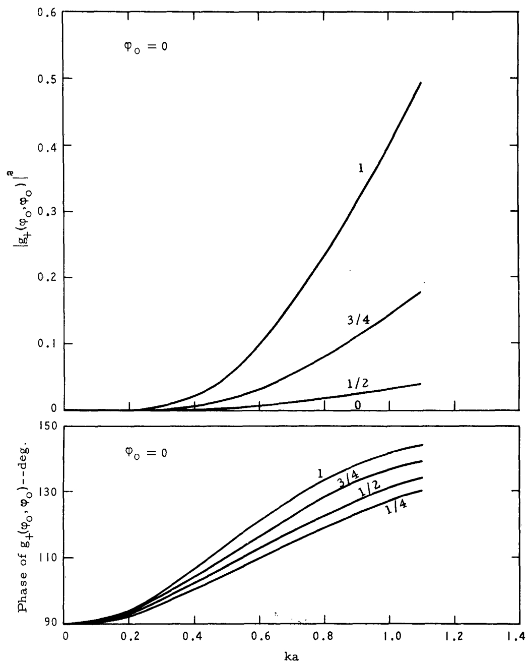
Graph I-3(a).
