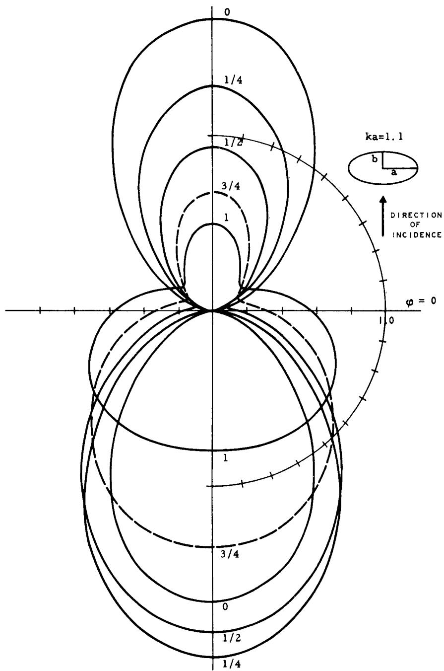
Graph I-10(c): |g_+(\varphi, 90^\circ)|^2 .
