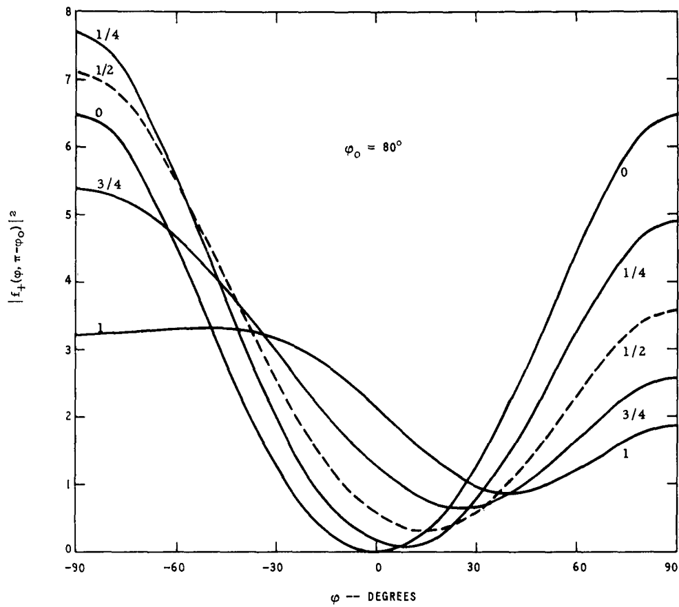
Graph III-8 (con't): ka = 1.1
