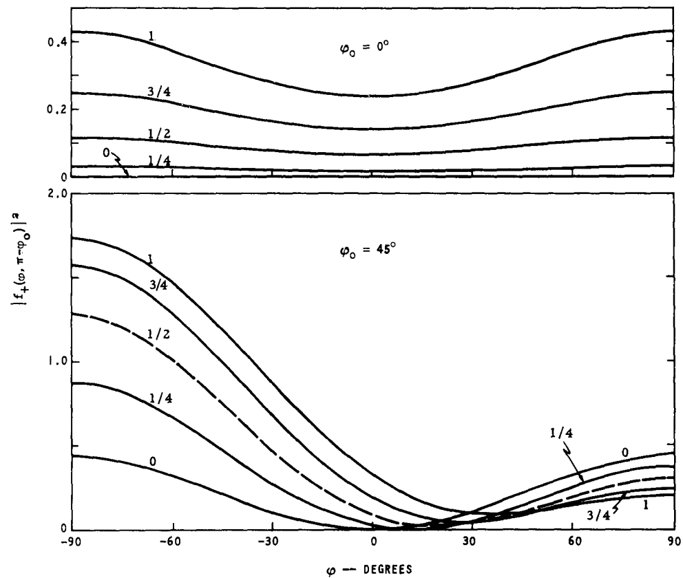
Graph III-7: ka = 0.7
