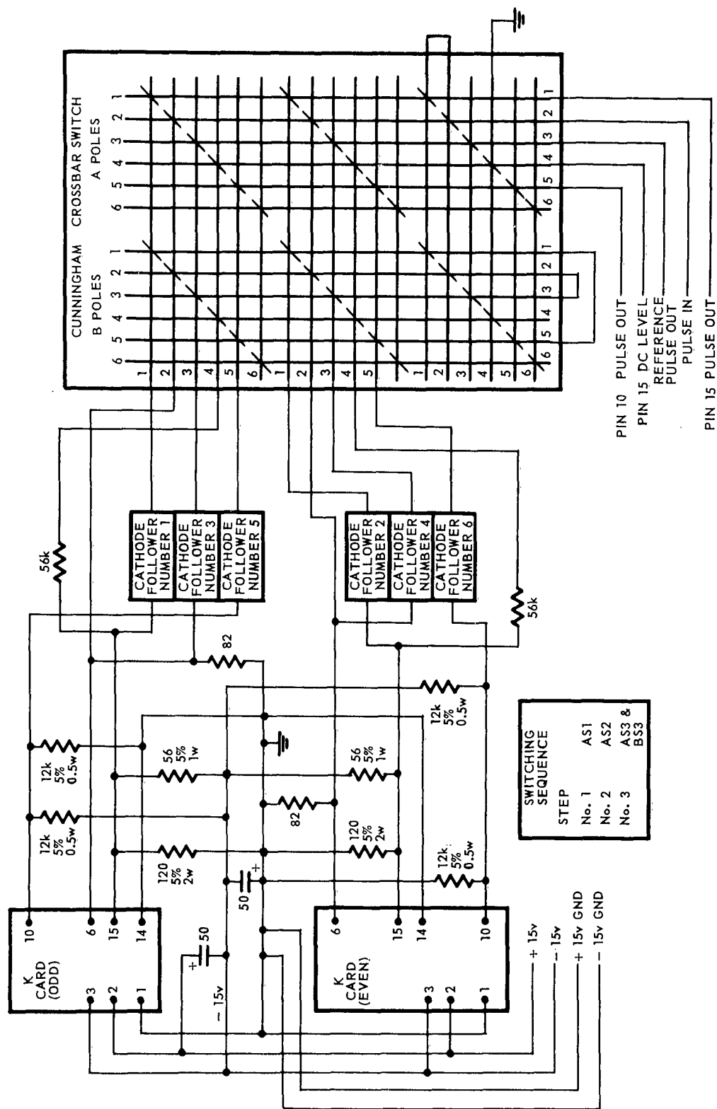
Figure 5-8 Type K Card Instrumentation
