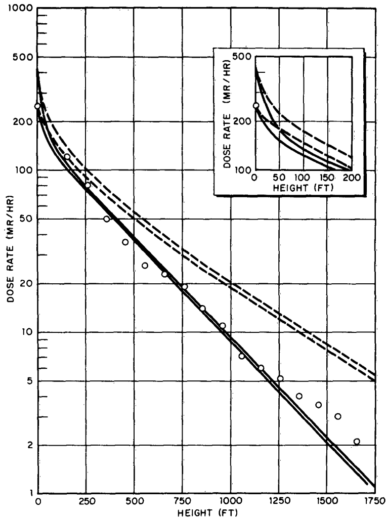
Fig. 2 Comparison of calculated and measured dose rate vs. height curves. The open circles are measured dose rates above a fallout field, 54-hr after the shot. The upper solid curve is the dose rate calculated from measurements of the gamma-ray energy spectrum and intensity of fallout collected from the same area in which the measurements were made. The lower solid curve is the same calculations shifted so as to correspond to ground roughness equivalent to 20 ft of air. The upper dashed curve is Spencer's dose vs. height (corrected for air density) curve for 1.12-hr fission products, and no ground roughness. It is normalized to Schuert's calculation at zero height. The lower dashed curve is Spencer's calculation adjusted to a ground roughness effect equivalent to \tau = 37 ft of air.
