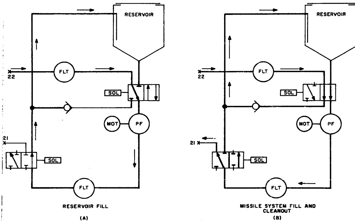
Figure 6-57. Power supply fill and filtering section - schema
