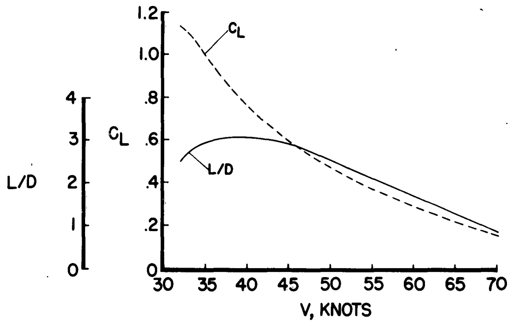
Fig.17 Longitudinal performance of the FRC paraglider
